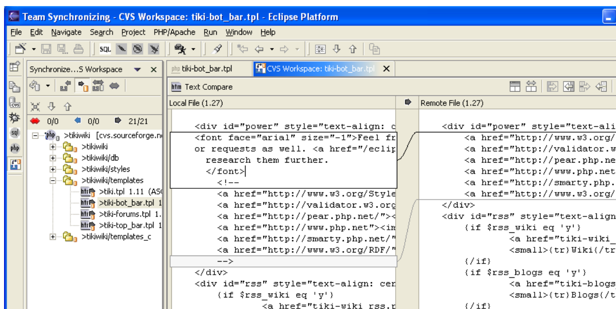
Comparing versions in Eclipse
