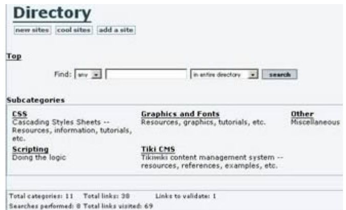
Browse_Directory
