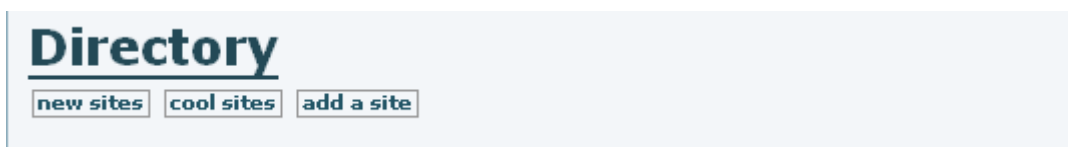
Navbar_links
